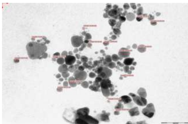
Fig 5: Transmission electron microscopic photographs of synthesized silver nanoparticles from Annona squamosa .
